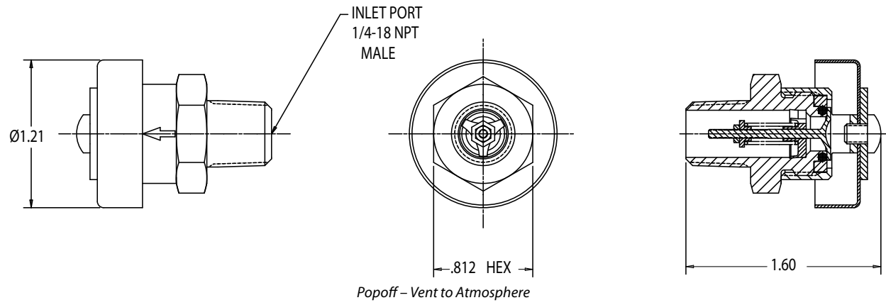
CSC L500-2MP Relief Valve (In-Line) Flow Data (ESR 21625)
